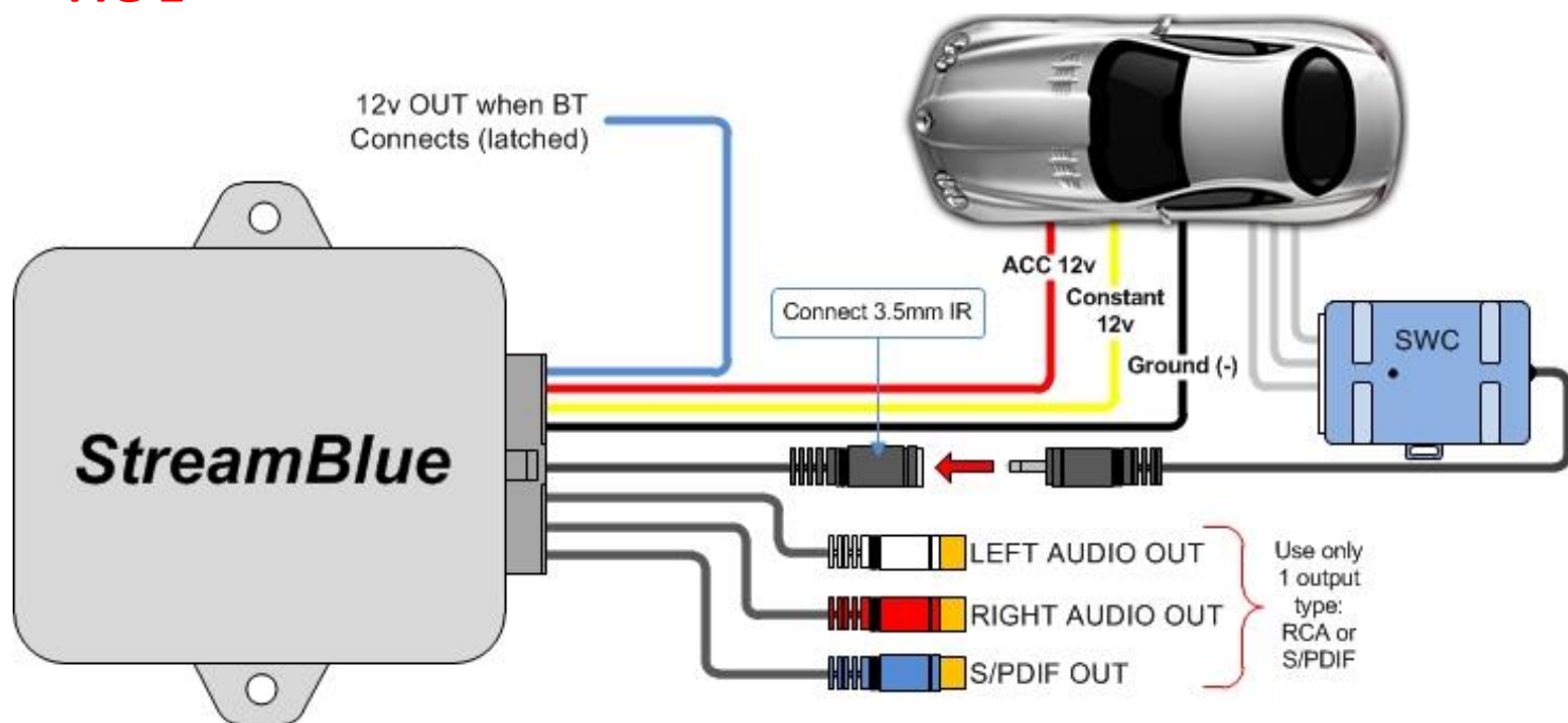
FIG 1 For adding Bluetooth and steering wheel controls (radio replaced with tablet)
