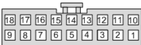
Wire side view
