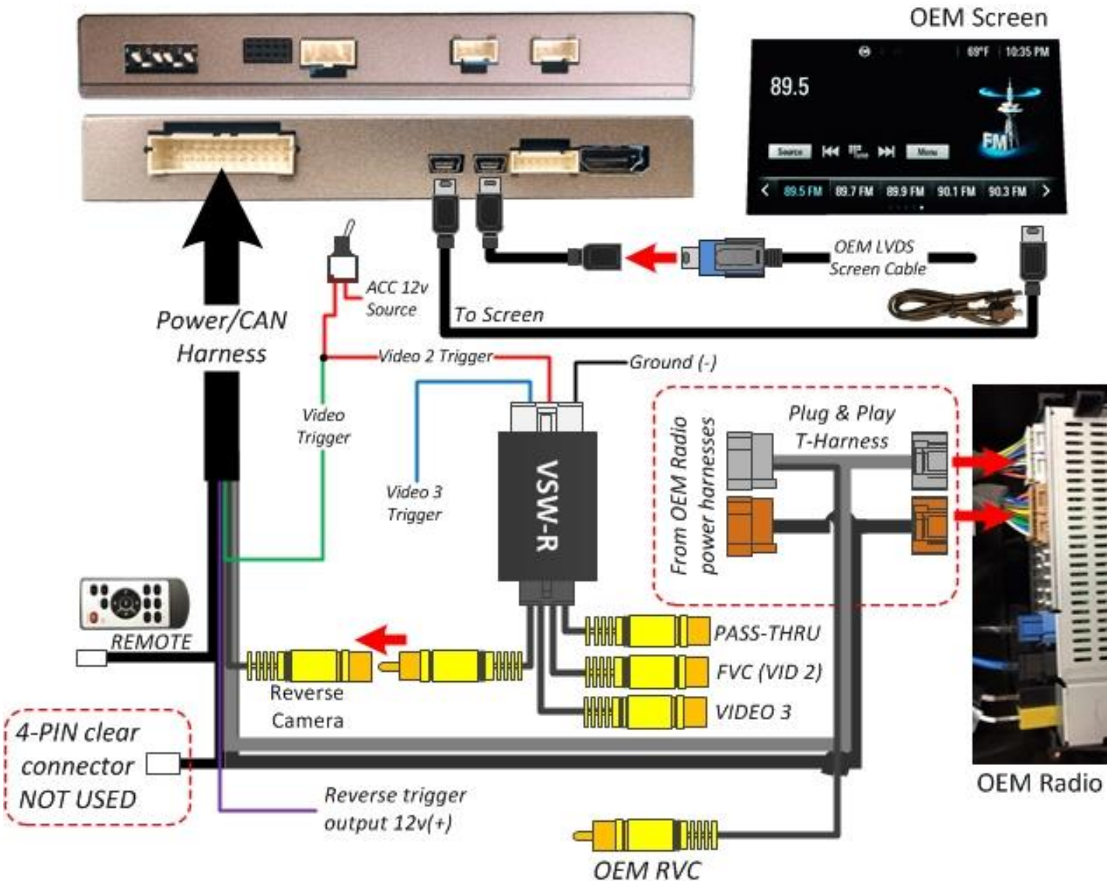
FIG 2: IOB-RVC Connection Diagram (adding FVC or AUX Video)
