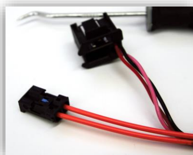
FIG 3: Fiber cable removed from factory plug
