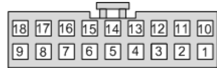
Wire Side
