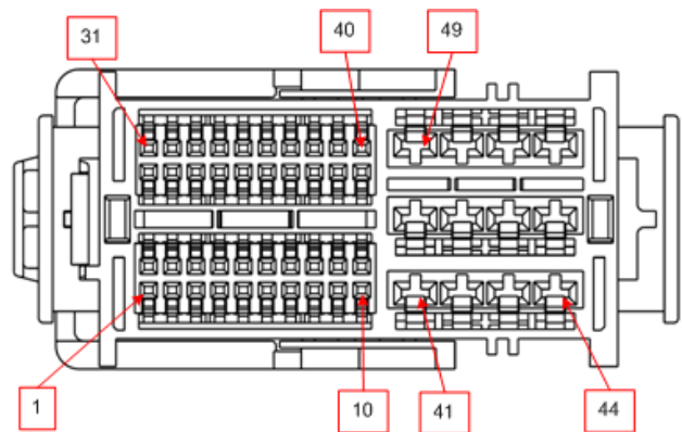
PIN Side
