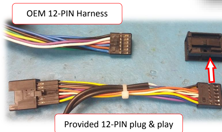
OEM 12-pin outer shell
