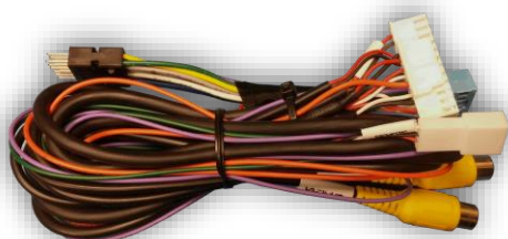
Power/CAN Harness
